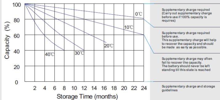
Storage characteristic
