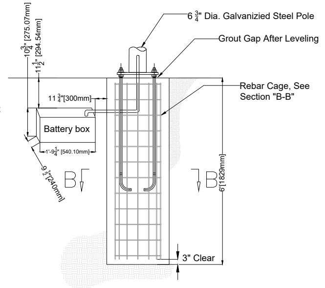
FOUNDATION SECTION
