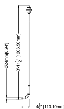
ANCHOR BOLT DETAIL
