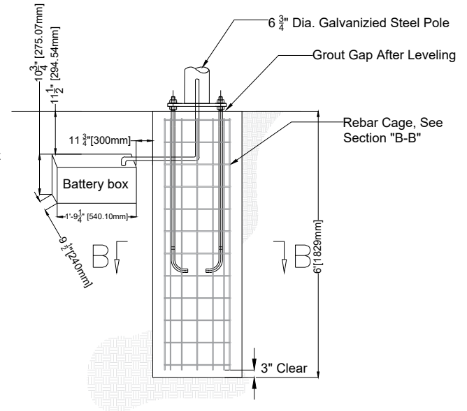
FOUNDATION SECTION
