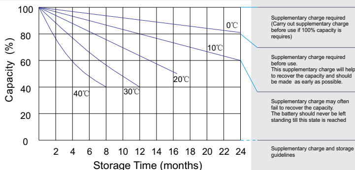
Storage characteristic
