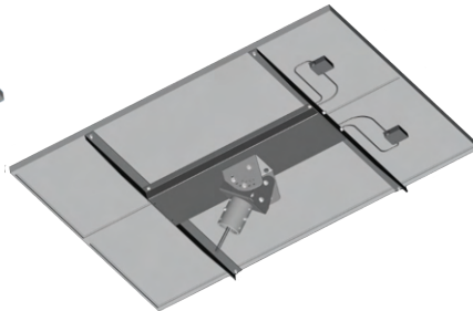
DUAL MOUNT
